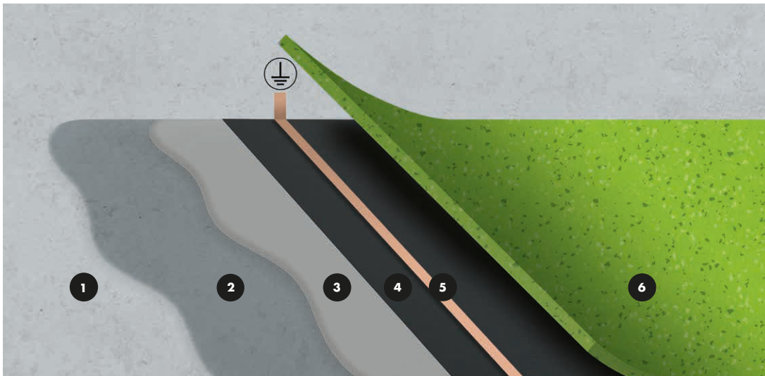
1 Substrate 2 Primer (where needed) 3 Leveler (where needed) 4 nora dryfix ed 5 Copper strip 6 nora ed floor covering
